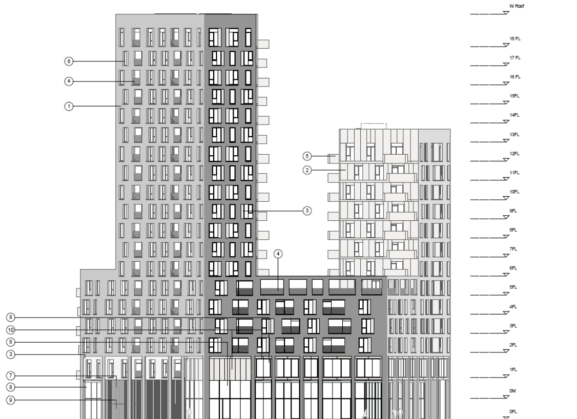
Image 1.15 – Ashley Road West – Proposed Southwest Elevation
