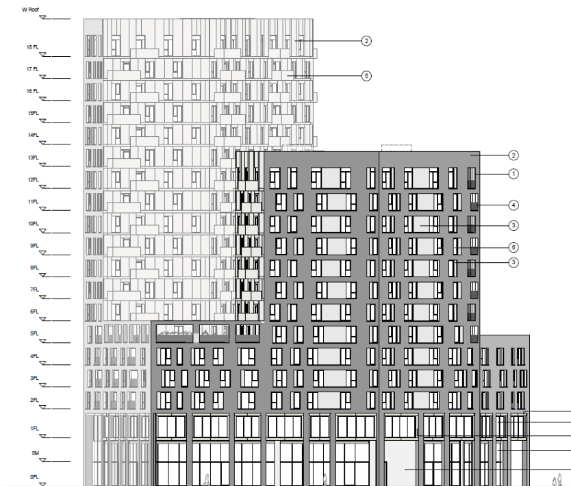
Image 1.15 – Ashley Road West – Proposed Southwest Elevation
