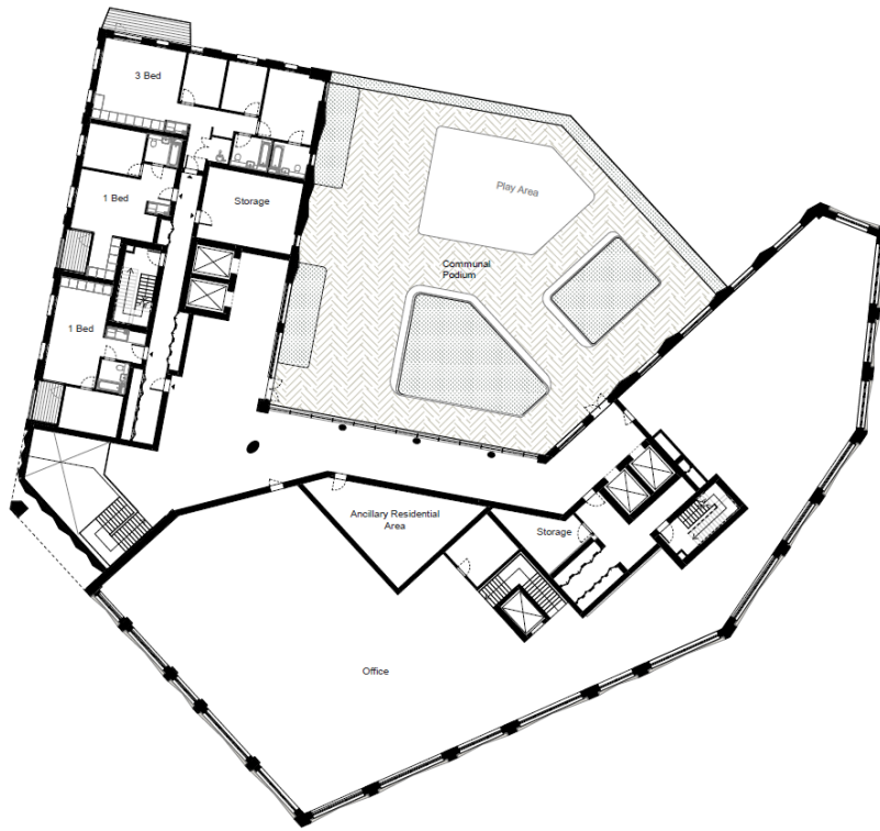
Image 1.3 – Ashley Road West – Proposed First Floor
