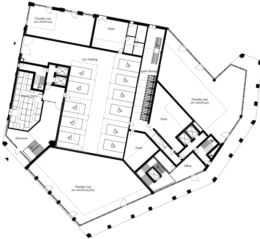
Image 1.1 – Ashley Road West – Proposed Ground Floor
