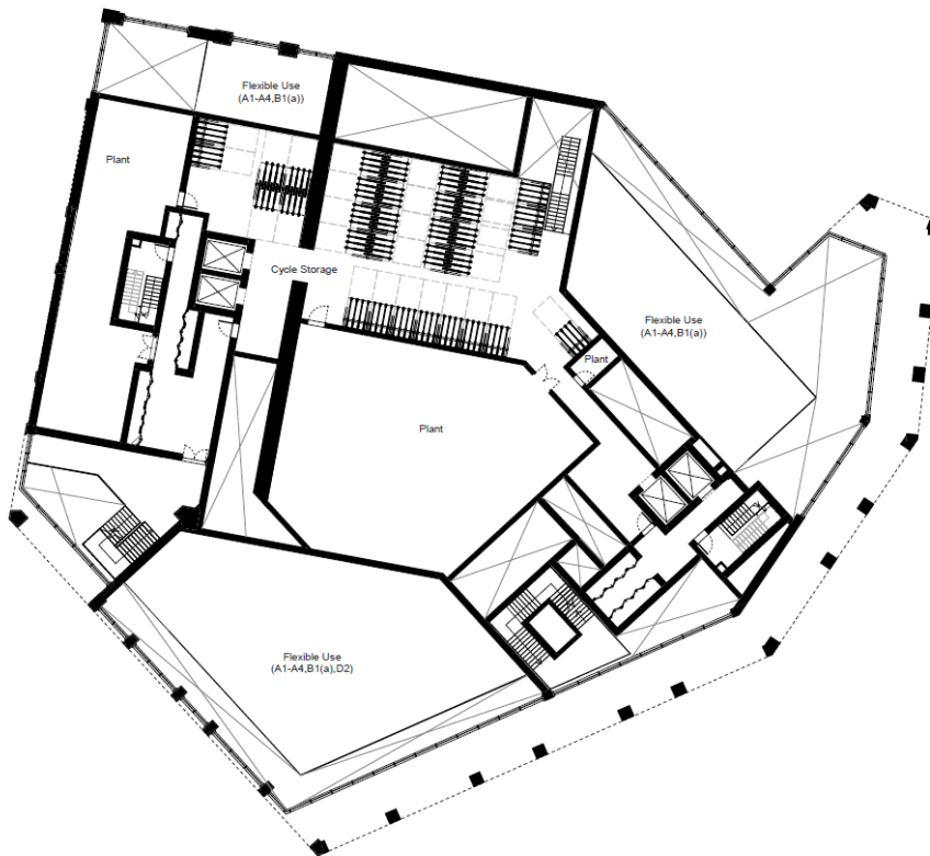
Image 1.2 – Ashley Road West – Proposed Mezzanine Floor
